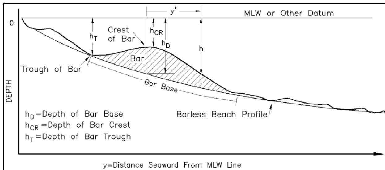
Figure III-3-12. Definition of offshore bar characteristics (Keulegan 1945)
