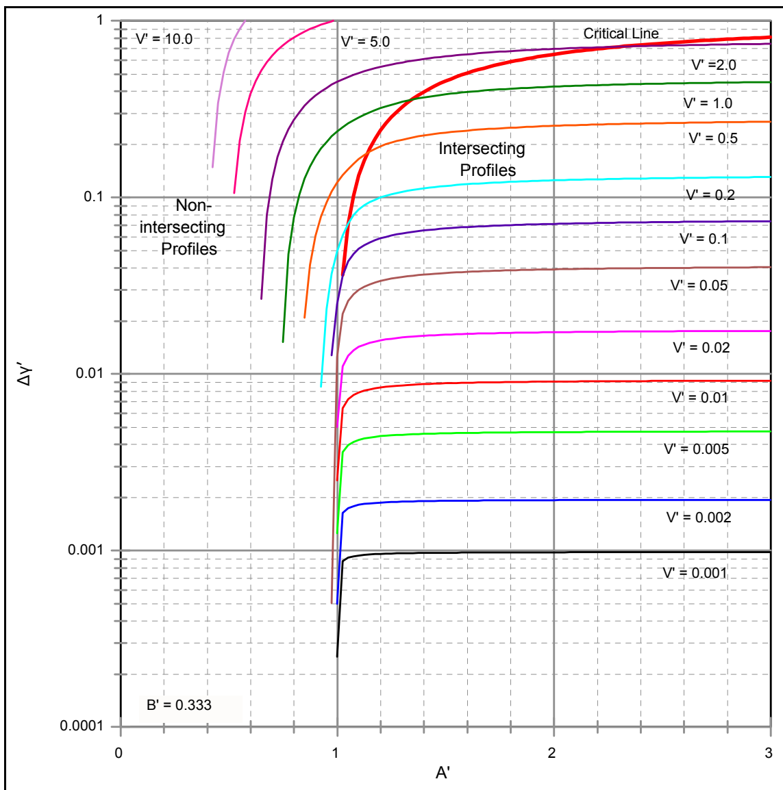
Figure III-3-25. Variation of nondimensional shoreline advancement \Delta y/W. , with A' and V' . Results shown for H/B = 3.0 ( B' = 0.333 ) (based on Dean (1991), values recomputed by Dean, May 2001). Intersecting and non-intersecting profiles divided by critical line; definition sketches shown in Figure III-3-20.
