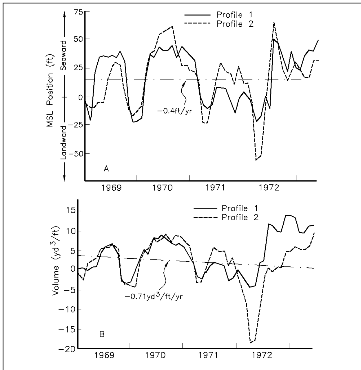
Figure III-3-30. Mean monthly shoreline position (A) and unit volume (B) at Jupiter Island, FL, referenced to first survey (Dewall and Richter 1977)
