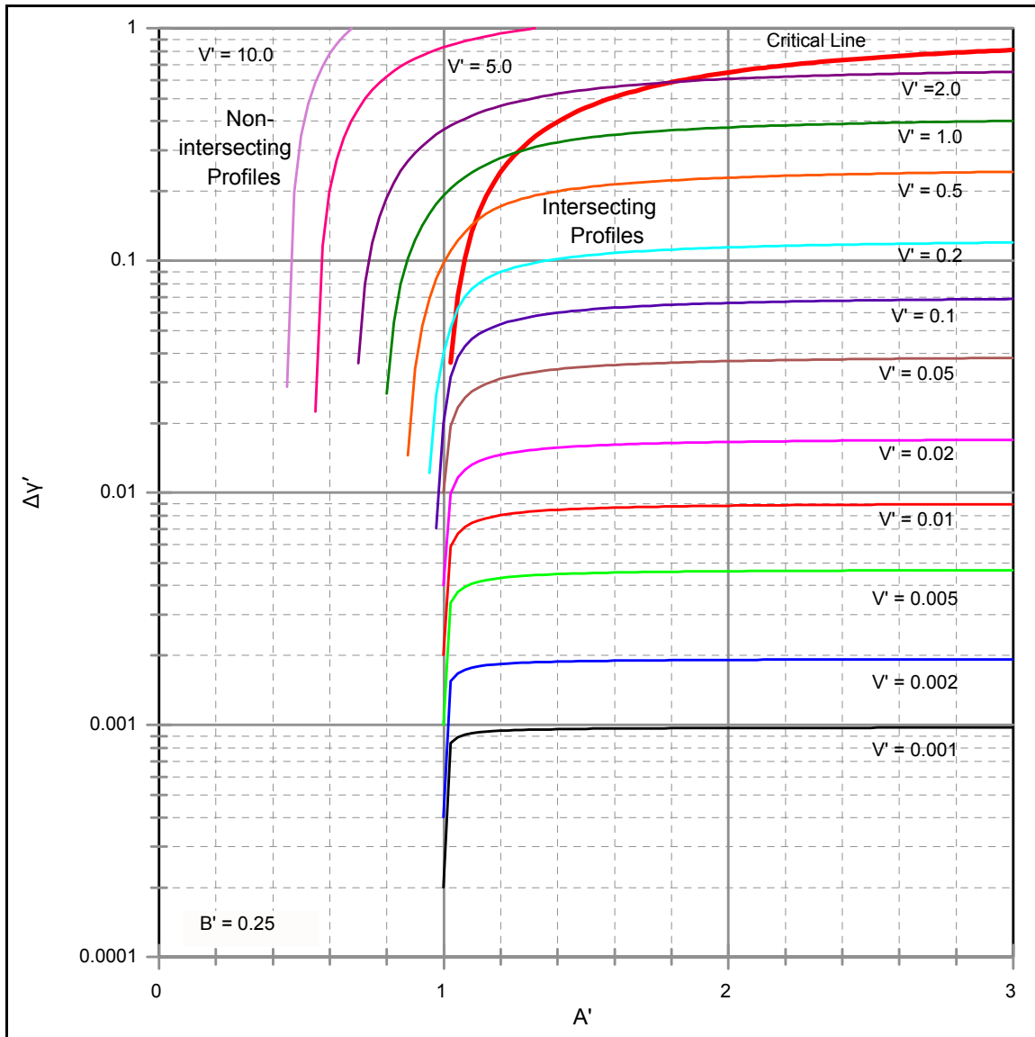
Figure III-3-26. Variation of nondimensional shoreline advancement \Delta y/W , with A' and V . Results shown for H/B = 4.0 ( B' = 0.25 ), based on Dean (1991), values recomputed by Dean, May 2001). Intersecting and non-intersecting profiles divided by critical line; definition sketches shown in Figure III-3-20.
