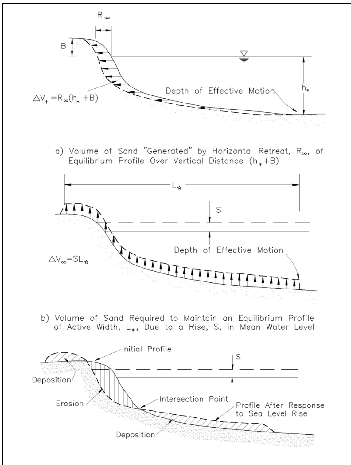
Figure III-3-32. Components of sand volume balance due to sea level rise and associated profile retreat according to the Bruun Rule
