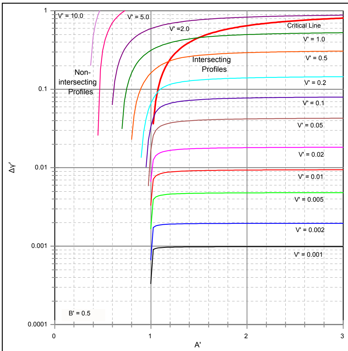
Figure III-3-24. Variation of nondimensional shoreline advancement \Delta y/W_* , with A' and V' . Results shown for H_o/B = 2.0 ( B' = 0.5 ) (based on Dean (1991), values recomputed by Dean, May 2001). Intersecting and non-intersecting profiles divided by critical line; definition sketches shown in Figure III-3-20.
