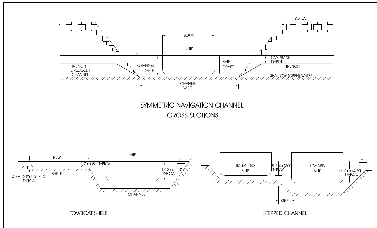
Figure V-5-16. Example channel cross sections
