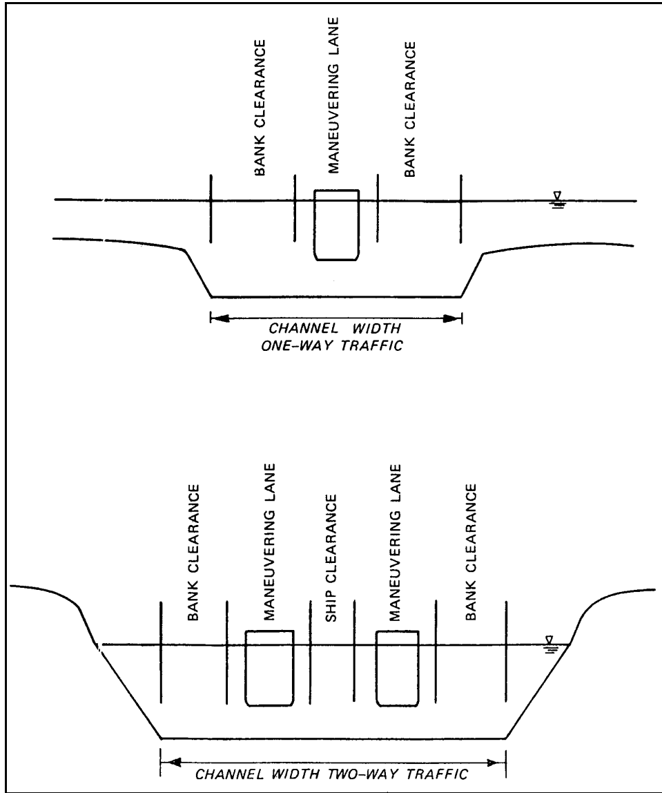
Figure V-5-24. Traditional interior channel width elements
