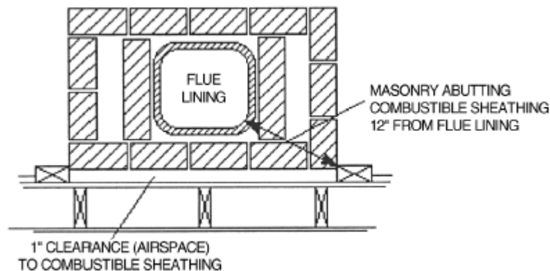
FIGURE 2113.19 ILLUSTRATION OF EXCEPTION THREE CHIMNEY CLEARANCE PROVISION
