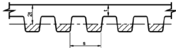
FIGURE 721.2.2.1.3 SLABS WITH RIBBED OR UNDULATING SOFFITS
