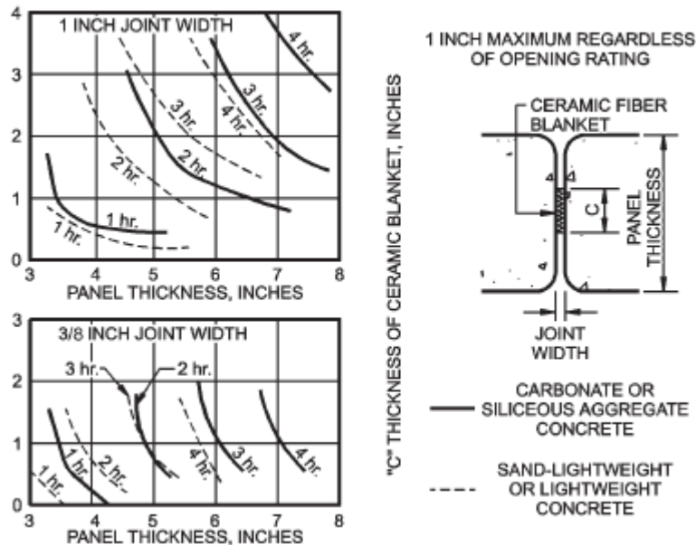
FIGURE 721.2.1.3.1 CERAMIC FIBER JOINT PROTECTION
