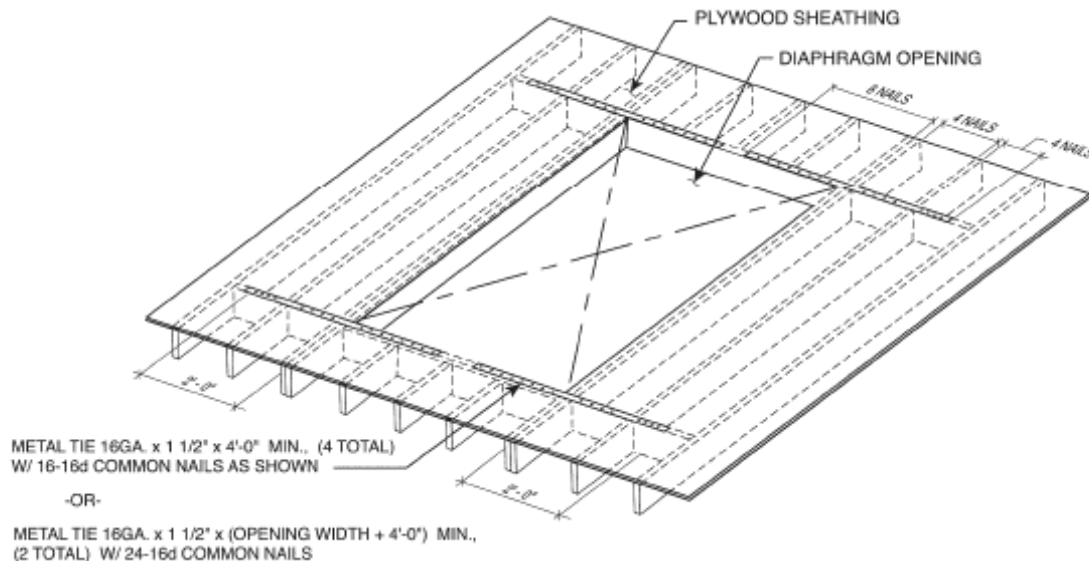
FIGURE 2308.11.3.3 OPENINGS IN HORIZONTAL DIAPHRAGMS
