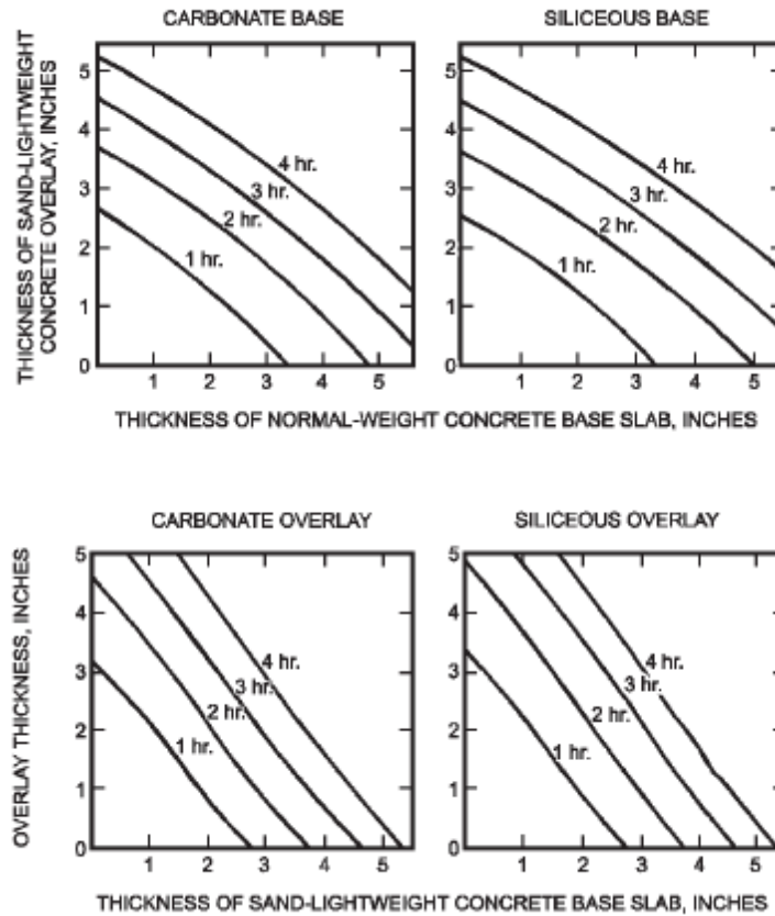
FIGURE 721.2.2.2 FIRE-RESISTANCE RATINGS FOR TWO-COURSE CONCRETE FLOORS
