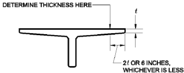
FIGURE 721.2.2.1.2 DETERMINATION OF SLAB THICKNESS FOR SLOPING SOFFITS
