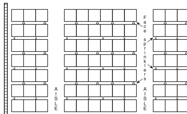
Elevation View
