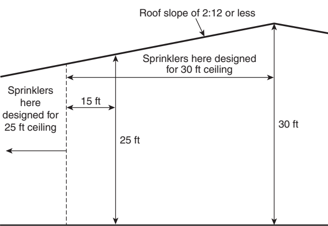
FIGURE A.12.1.3.1.4 Extended Sprinkler Coverage Under Sloped Ceilings.
