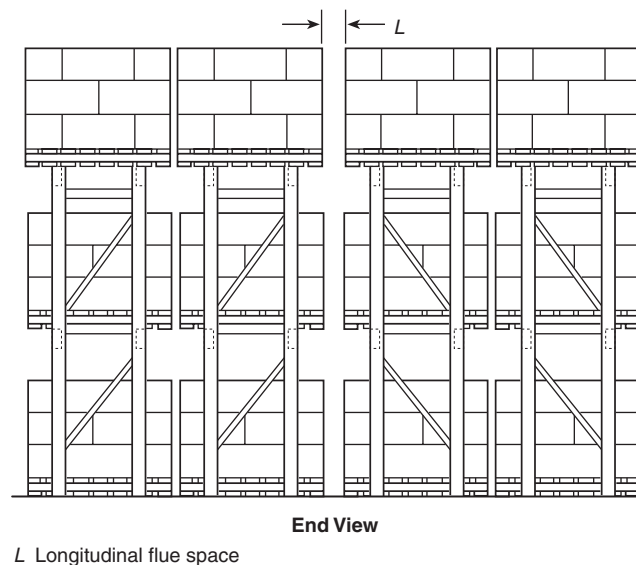
FIGURE A.3.9.3.7(f) Multiple-Row Rack Served by Reach Truck.
