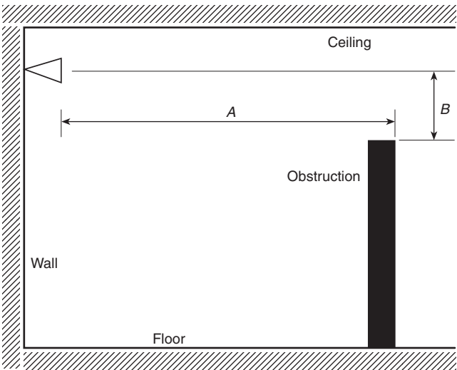
Elevation View
