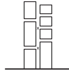
FIGURE A.16.3.1.3.1.1 Placement of In-Rack Sprinklers Where Rack Levels Have Varying Heights.
