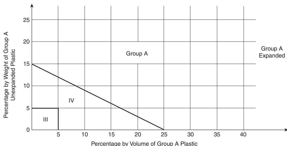
FIGURE 5.6.3.3.3(a) Commodities Containing a Mixture of Expanded and Unexpanded Group A Plastics.
