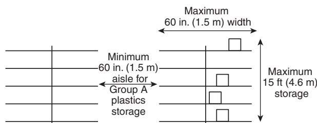
FIGURE A.3.9.2.6.1 Back-to-Back Shelf Storage.
