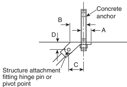
FIGURE A.9.3.5.12.2(a) Dimensions of Concrete Anchor for Orientations A, B, and C.
