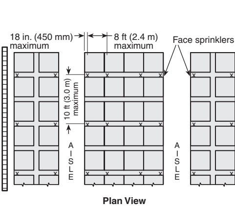
FIGURE 17.3.1.5(b) In-Rack Sprinkler Arrangement, Group A Plastic Commodities, Storage Height Over 25 ft (7.6 m) — Option 2.
