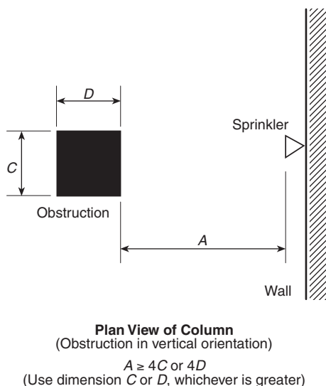
FIGURE 8.10.7.2.1.4(a) Minimum Distance from an Obstruction in the Vertical Orientation (Residential Sidewall Sprinkler).
