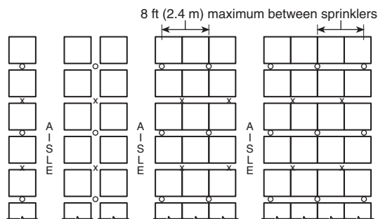
Plan View
