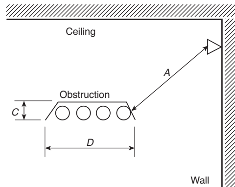
FIGURE 8.7.5.2.1.3(a) Minimum Distance from an Obstruction in the Vertical Orientation (Standard Sidewall Spray Sprinklers).
