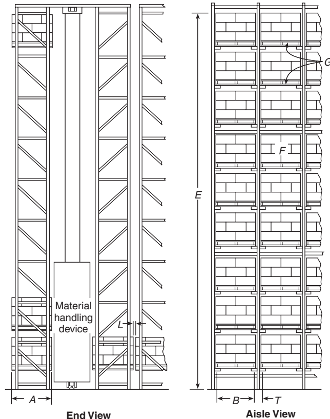
FIGURE A.3.9.3.7(c) Double-Row Racks with Solid Shelves.
