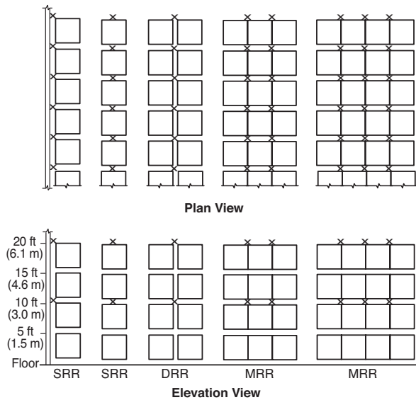
FIGURE 17.2.1.4(i) Exposed Nonexpanded Group A Plastics Up to 20 ft (6.1 m) in Height in Up to a 30 ft (9.1 m) High Building with One Level of Closely Spaced In-Rack Sprinklers.
