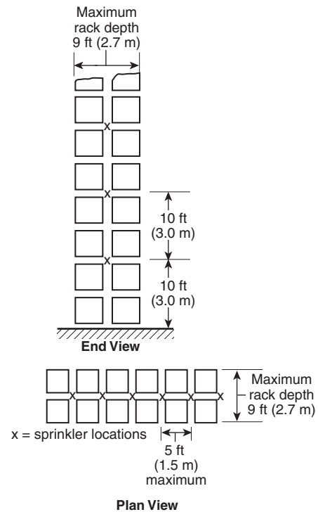
FIGURE 17.3.1.7 In-Rack Sprinkler Arrangement, Cartoned Expanded and Nonexpanded Group A Plastic and Exposed Non-expanded Group A Plastic Commodities, Single- and Double-Row Racks, Storage Height Over 25 ft (7.6 m).
