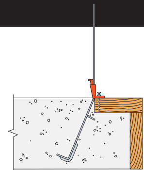
Alternate StrapMate Installation for Brick Ledges
