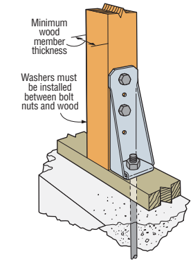
HD3B Vertical Installation
