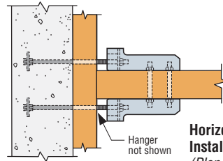
HD5B (HD7B and HD9B similar) U.S. Patents 6,006,487; 6,327,831
