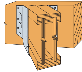
Typical HSUR4.12/9 Installation
