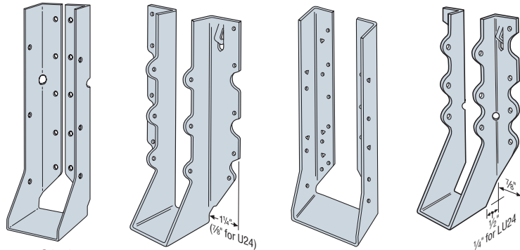
LUC210Z (LUC26Z Similar) U210 HUC412 Concealed Flanges LU28 (except LU Roughs)
