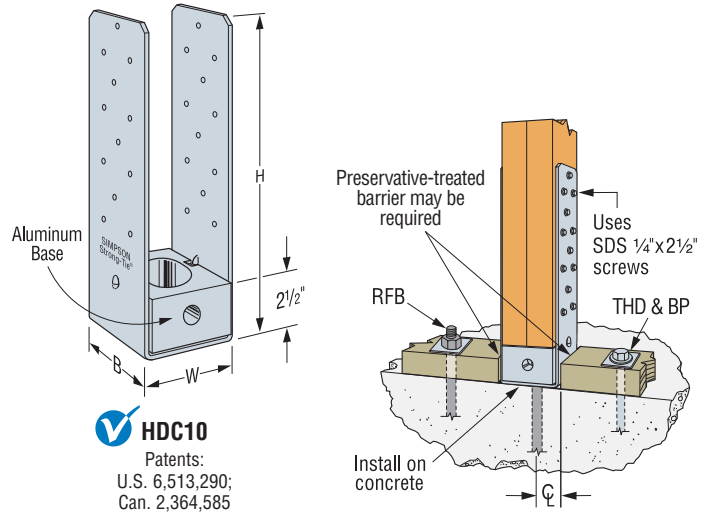
Typical HDC Installation with 2-2x4 Studs (Similar with 2-2x6 studs)
