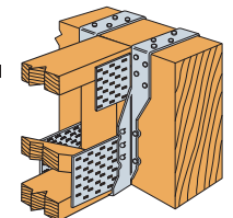
Alternate Installation of THA422
