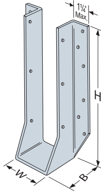
LUC210Z (LUC26Z Similar) U210 HUC412 Concealed Flanges LU28 (except LU Roughs)
