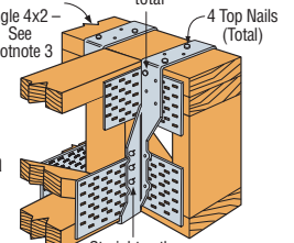
Typical THA422 Top Flange Installation on a 4x2 Floor Truss
