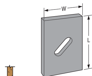
BPS \frac{1}{2} -6 (Other models similar)
