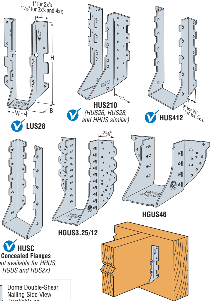
Typical LUS28 Installation use 0.148x3" (10d common) or 0.148x3 3/4" (16d sinker) nail
