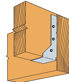
Typical HUCQ Installed on End of a Beam
