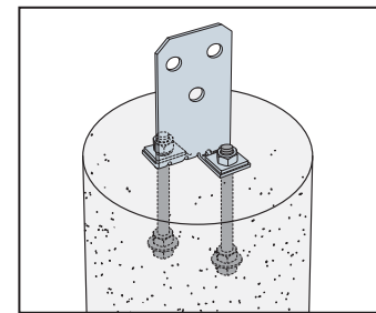
Circular Pedestal Installation
