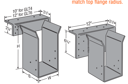
GLT (fasteners included) See pages 104-105 for GLT and HGLT information. HGLT (fasteners included)
