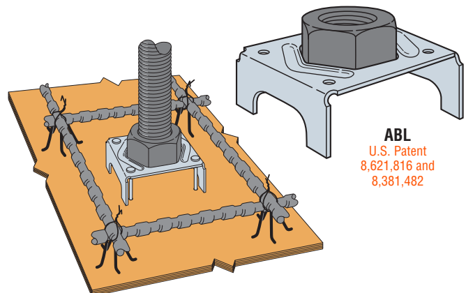
Typical ABL Installation
