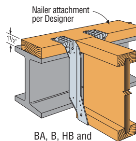
BA, B, HB and LBV are acceptable for nailer applications (BA shown on 2x nailer)
