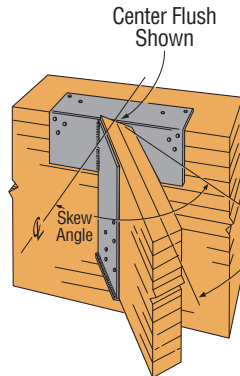
Typical GLT Sloped Down, Skewed Right
