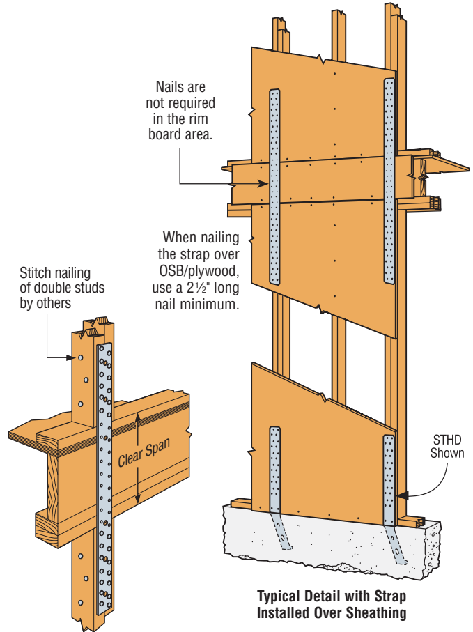
Floor-to-Floor Tie Installation showing a Clear Span
