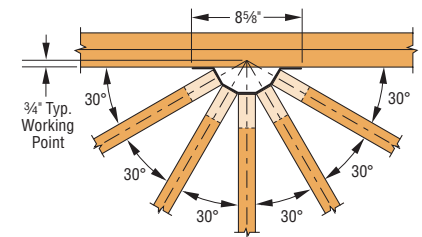
THJM2-5-SDS3 Top View Installation
