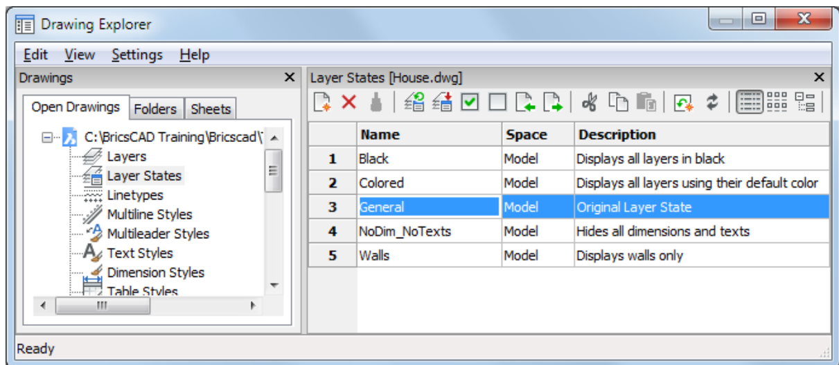
Drawing Explorer: Layer States (Detail view)
