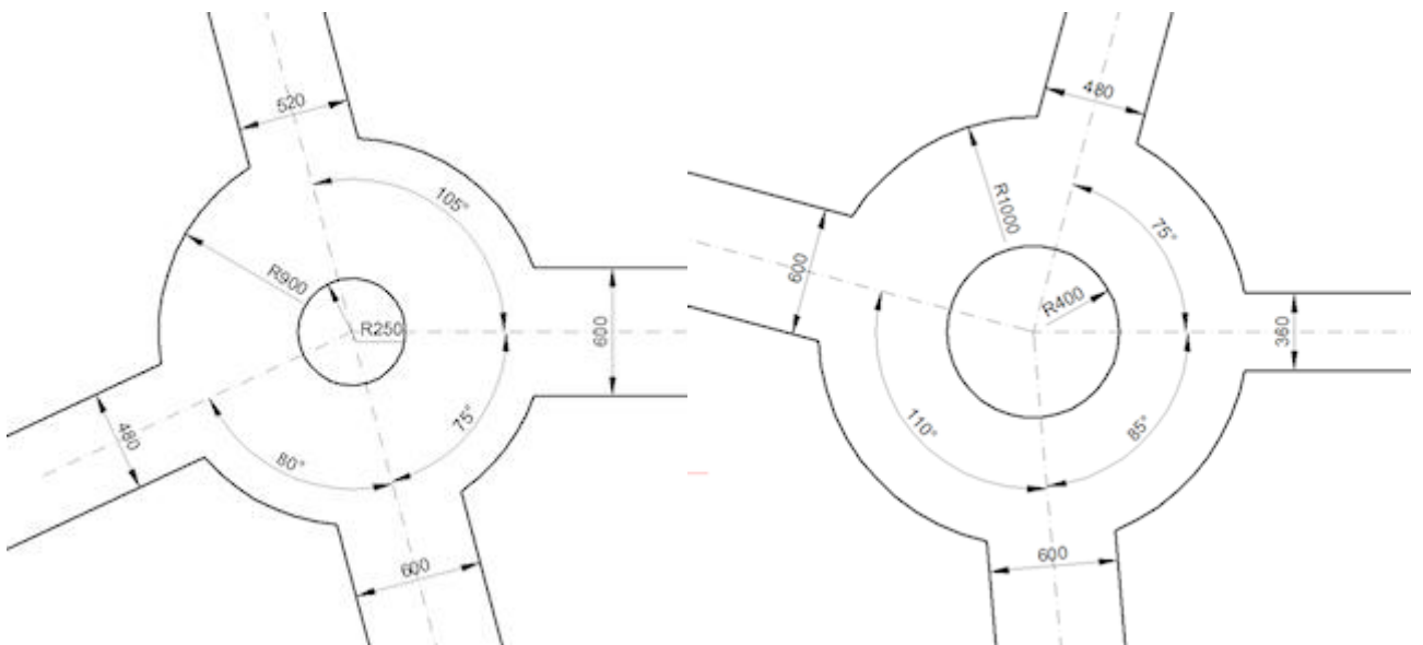
Two versions of the same fully constrained drawing representing a roundabout
