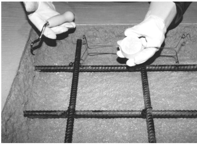
Fig. 6—Tying tool and Type 1A anode.
