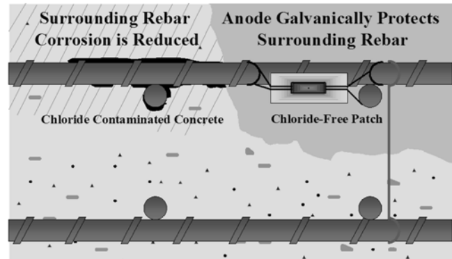
Fig. 2—Chloride-accelerated corrosion.
