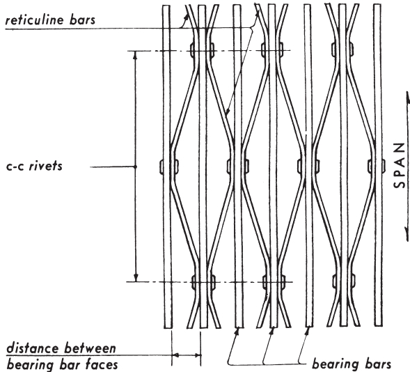
RIVETED GRATING
