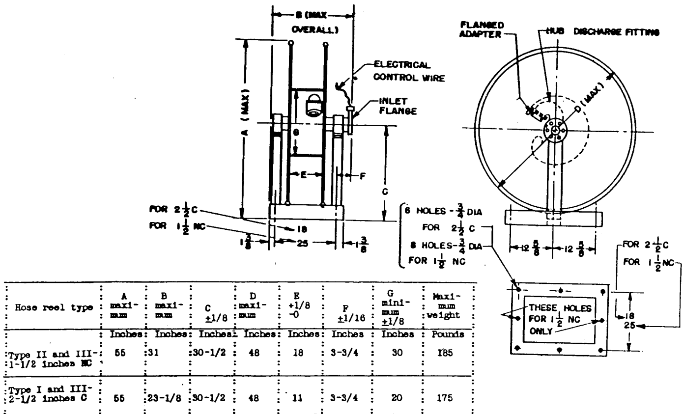
FIG. 1 Hose Reel Dimensions
