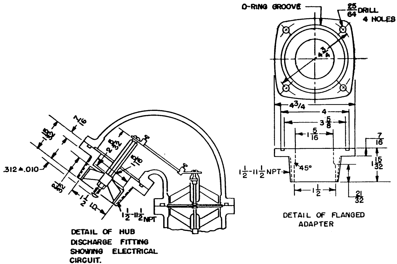
FIG. 3 Discharge Fitting and Adapter Details for Type 2 and 3, 1 1/2-in. (38-mm) Noncollapsible Reels
