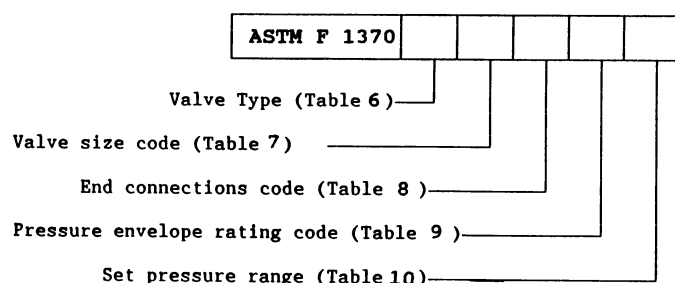
FIG. 1 Valve Coding System
