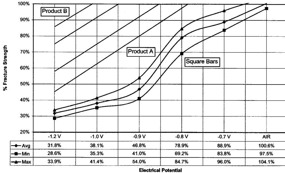
FIG. X1.2 Threshold Determination Product Versus Sq(B)s
