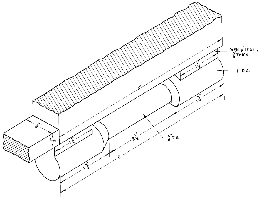
(b) Design of the Vertical Grip-Web Bar (Gating and Rising System as in ( a))
