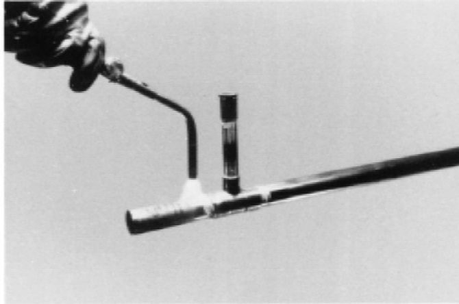
FIG. 15 Preheating: Tube
