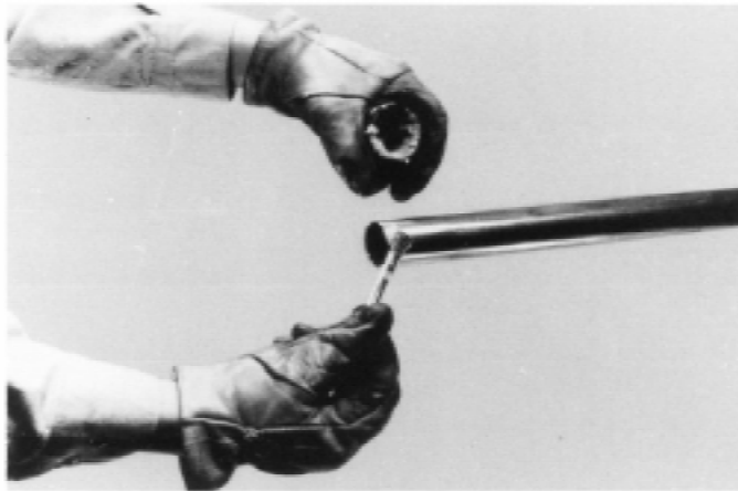
FIG. 10 Fluxing: Tube
