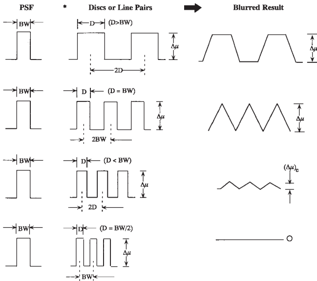
FIG. 17 An Illustration of a One-Dimensional Profile Through the Center of Periodic Features of Varying Diameters Which Have Been Convolved With a CT PSF: (a) D > BW , (b) D = BW , (c) BW/2 < D < BW , and (d) D = BW/2
