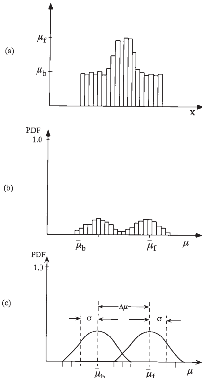
FIG. 19 (a) A Line Profile Through the Center of a Noisy Feature Convolved With a CT PSF and Pixelized; (b) A Probability-Distribution Function for the Profile in (a); and (c) A Continuous Representation of the PDFs of (b) With the Means, Standard Deviations, and Contrast Difference Indicated
