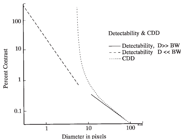
FIG. 20 A Plot Illustrating the Application of the Detectability Lines and the CDD Curve for a Cylinder of Iron of Radius 2.54 cm that is Irradiated By 0.8-MeV X-Ray Photons: A Value of 8.5 was used for the Constant c in Eq 25 and its Derivative Equations
