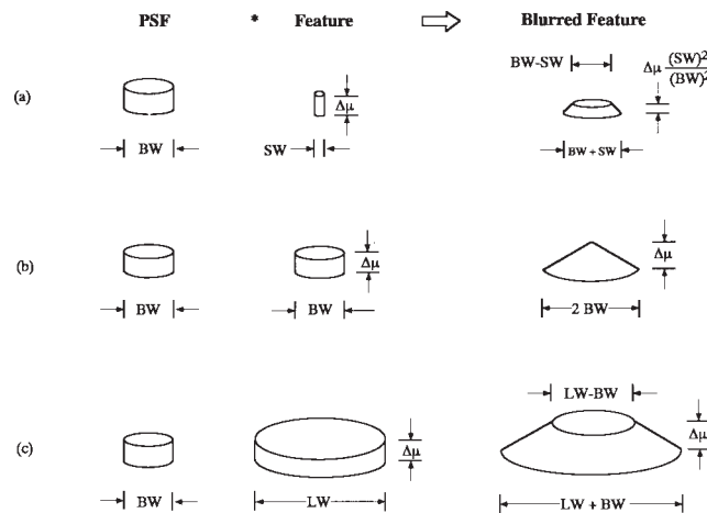
FIG. 15 A Sketch Illustrating the Two-Dimensional Convolution of a Point-Spread Function (PSF) of Diameter BW with Features of Varying Diameters: (a) SW < BW , (b) BW = BW , and (c) LW > BW . The Symbol (*) Represents the Convolution of Two Functions
