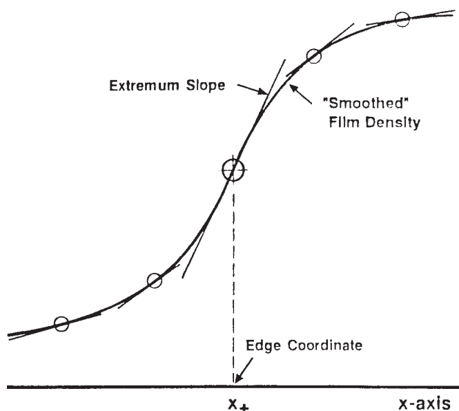
FIG. 3 Depiction of Various Slopes on a Smoothed Microdensitometer Trace; The Object Edge Coordinate, x_+ , Corresponds to the Extremum Slope Point on the Trace
