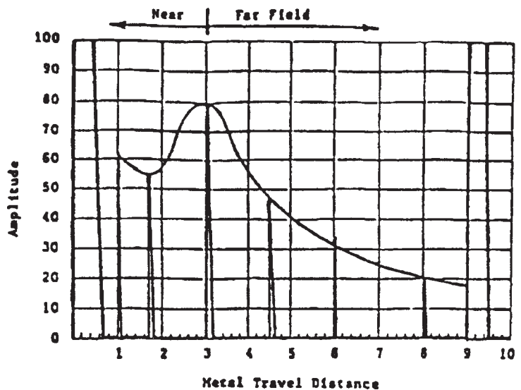
FIG. 1 Typical Calibration Curve
