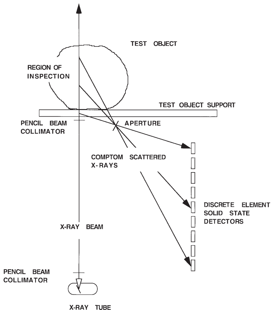
FIG. 9 General Arrangement of X-Ray Source, Detector Array and Test Object for a Simultaneous Multi-Plane Compton Tomographic Imaging System
