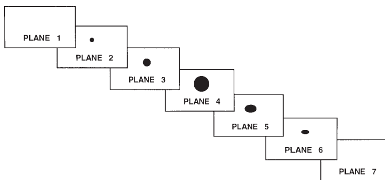
FIG. 7 Simulated CST Image Display of a Homogenous Test Object Containing a Void
