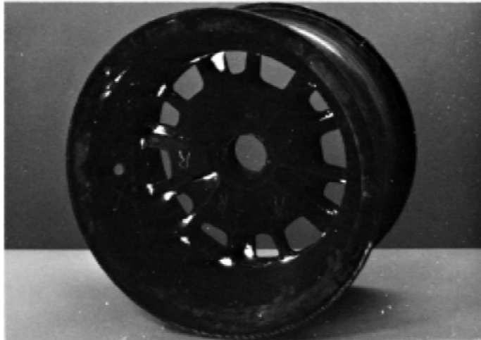
FIG. 4 Example of Type I, Class D, Indication
