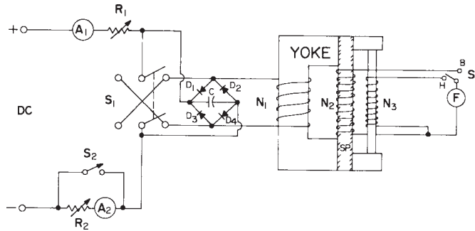
FIG. X6.1 Schematic Illustration of Arc Suppression Diode Bridge Placed in the Circuit Shown Previously in Fig. 1
