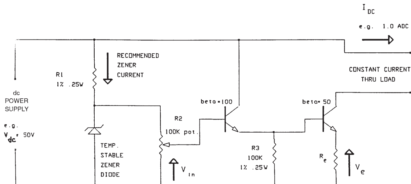
FIG. 4 Typical Constant dc Source
