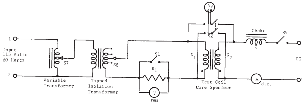
FIG. 2 Basic Circuit for the Measurement of Impedance and Incremental Permeability and the Apparent A-C Magnetizing Force
