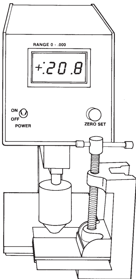
NOTE 1—The amorphous strips extend over the anvil of the micrometer. FIG. X1.2 Holding Fixture in Position for Thickness Measurement
