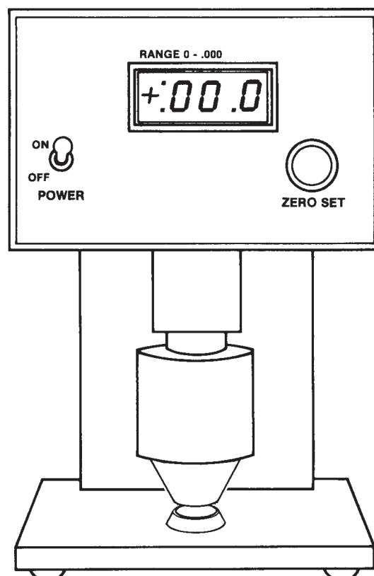
FIG. X1.1 Automatic Digital Micrometer for Thickness Measurement
