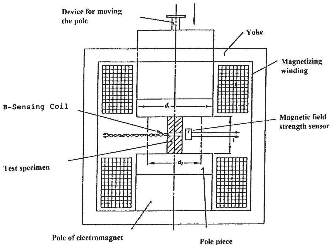
FIG. A1.1 Diagram of an Electromagnet
