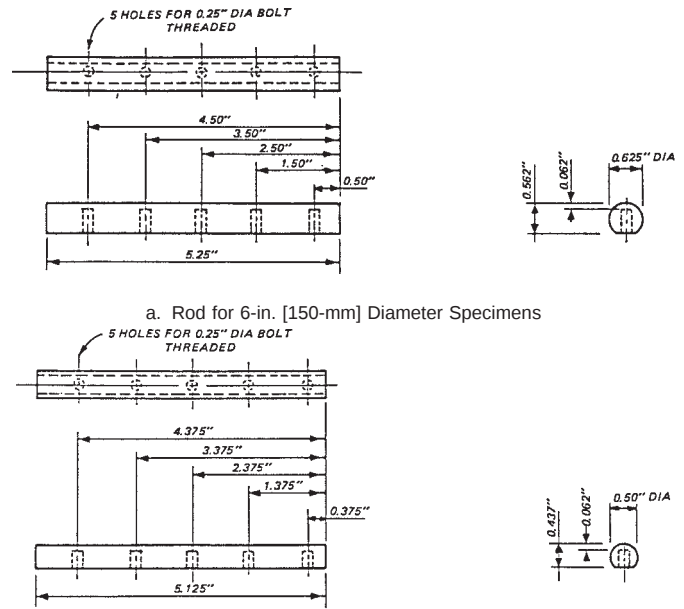
b. Rod for 4-in. [100-mm] Diameter Specimens
