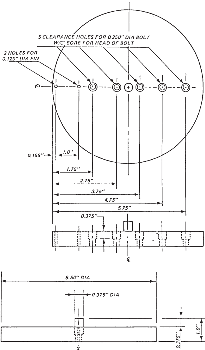
FIG. 3 Base Plate
