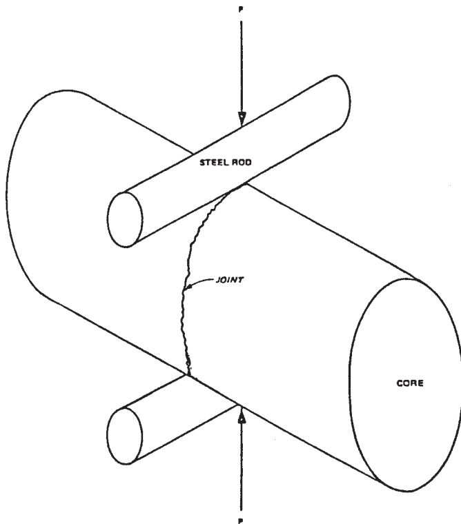
FIG. 1 Schematic of Loading Method
