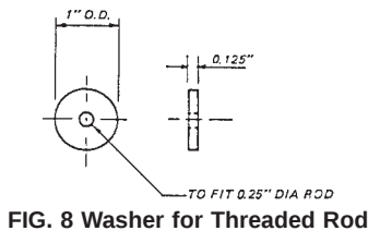
FIG. 8 Washer for Threaded Rod
