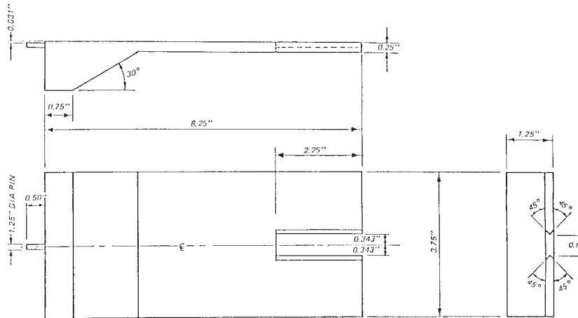
FIG. 10 Alignment Post for 6-in. [150-mm] Diameter Specimens
