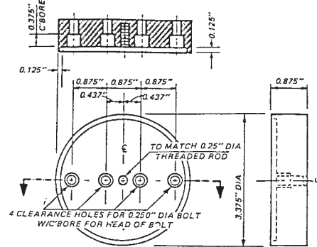
FIG. 5 Top Plate
