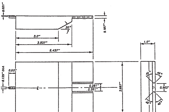
FIG. 9 Alignment Post for 4-in. [100-mm] Diameter Specimens
