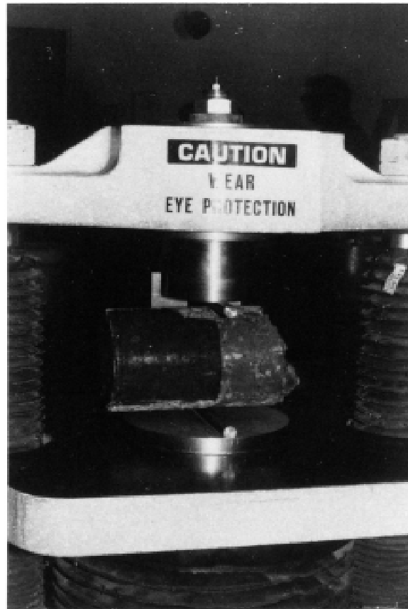
FIG. 2 Test Specimen in Testing Machine
