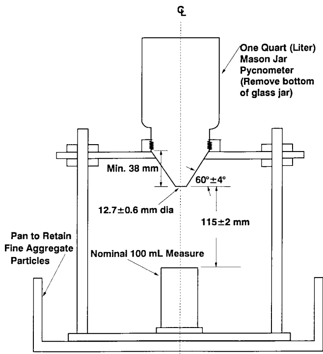
Section Through Center of Apparatus
