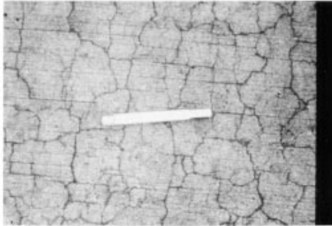
FIG. X2.44 Low-Severity Crazing
