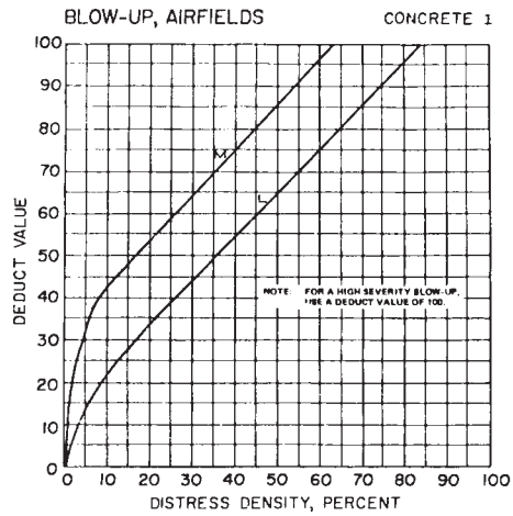
FIG. X4.1 Blowup
