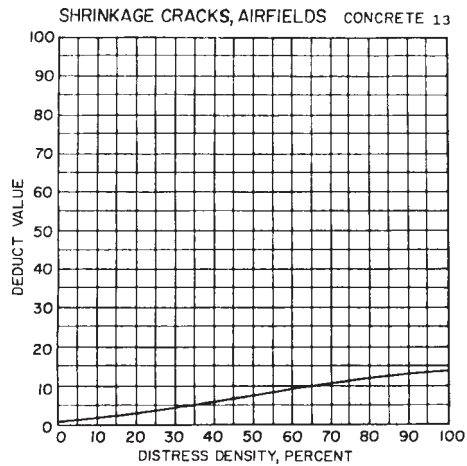
FIG. X4.13 Shrinkage Cracking
