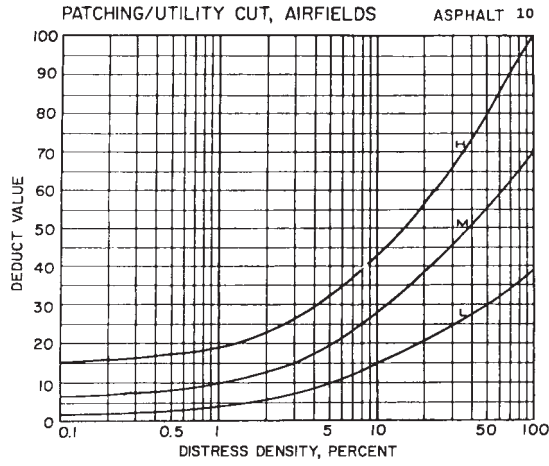
FIG. X3.12 Patching
