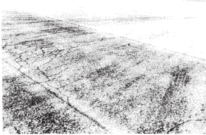
FIG. X1.8 Medium-Severity Alligator Cracking, Approaching High Severity (Example 2)
