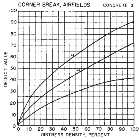
FIG. X4.2 Corner Break
