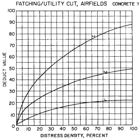
FIG. X4.7 Patching/Utility Cut
