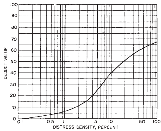
FIG. X3.2 Distress 2, Bleeding
