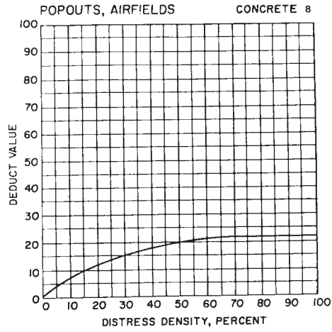
FIG. X4.8 Popouts
