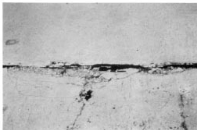
FIG. X2.67 High-Severity Joint Spall
