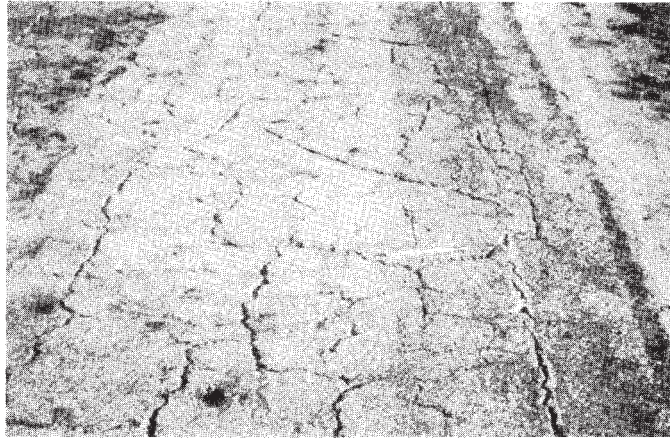
FIG. X1.20 High-Severity Block Cracking
