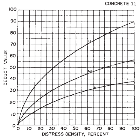
FIG. X4.11 Faulting
