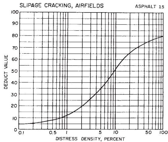
FIG. X3.17 Slippage Cracking
