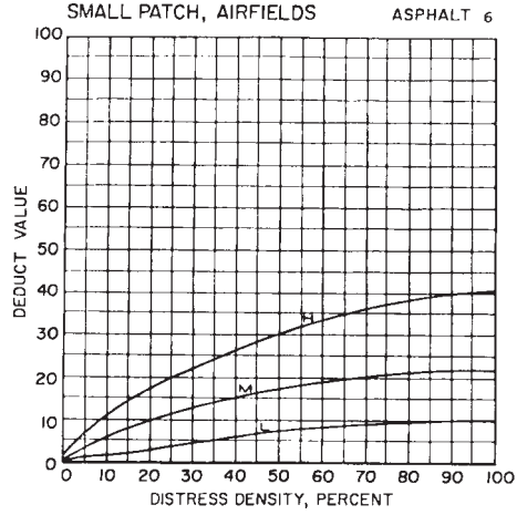
FIG. X4.6 Small Patch
