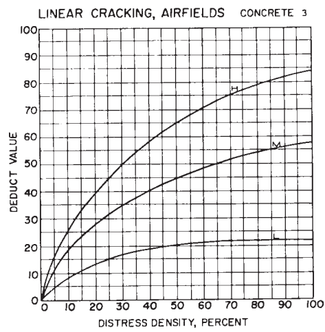
FIG. X4.3 Linear Cracking
