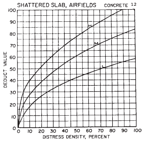
FIG. X4.12 Shattered Slab
