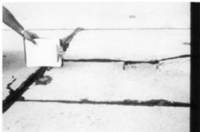
FIG. X2.49 Low-Severity Settlement (3/8 in. (9 mm)) on Apron
