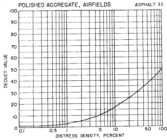
FIG. X3.13 Polished Aggregate
