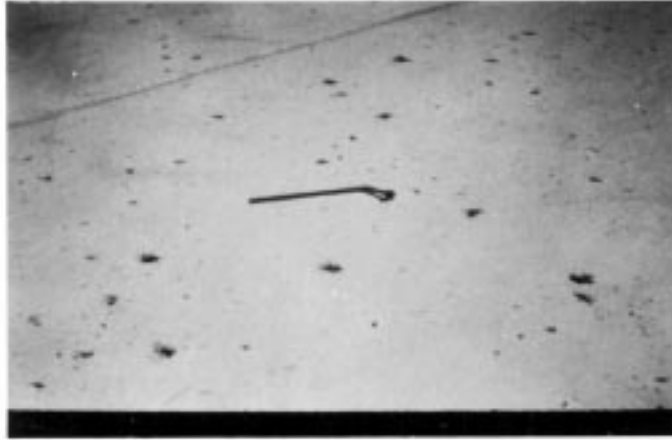
FIG. X2.38 Popouts
