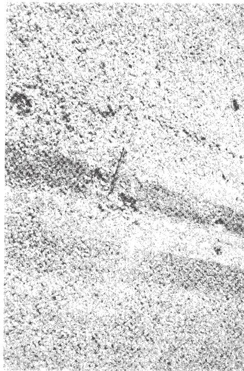
FIG. X1.65 High-Severity Raveling/Weathering on a Porous Friction Course Surface
