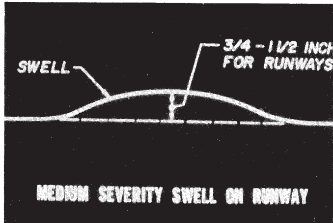
FIG. X1.76 Medium-Severity Swell
