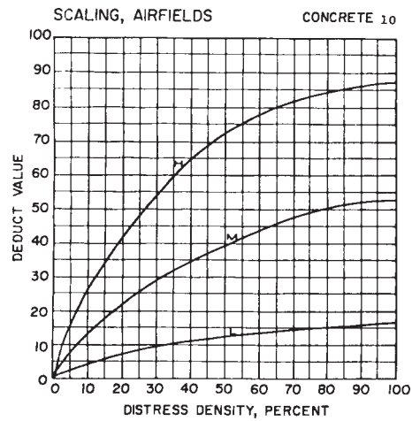
FIG. X4.10 Scaling/Crazing
