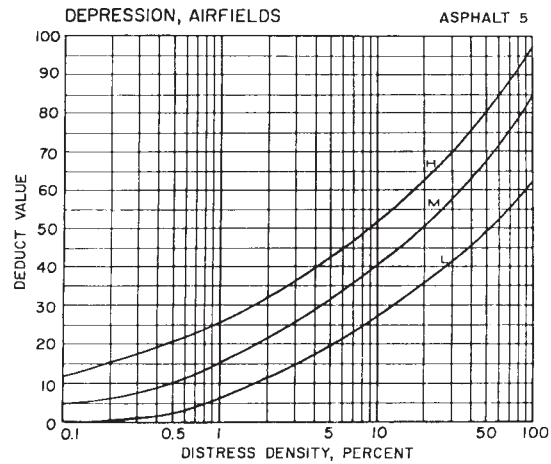
FIG. X3.5 Depression
