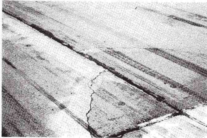
FIG. X2.7 Medium-Severity Corner Break
