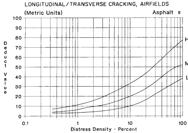
FIG. X3.10 Longitudinal/Transverse Cracking (Metric)
