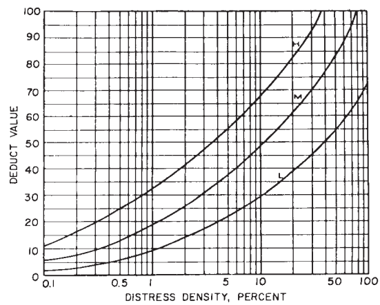
FIG. X3.4 Distress 4, Corrugation
