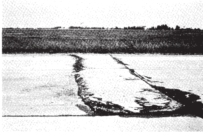
FIG. X2.2 Medium-Severity Blowup
