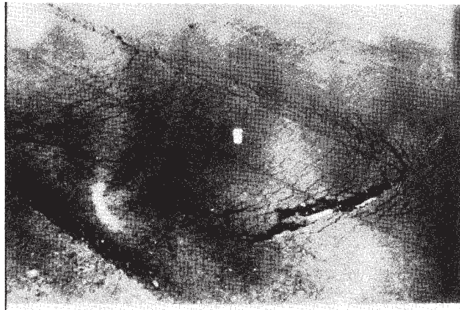
FIG. X1.74 Slippage Cracking
