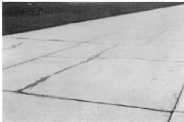
FIG. X2.57 Medium-Severity Intersecting Cracks
