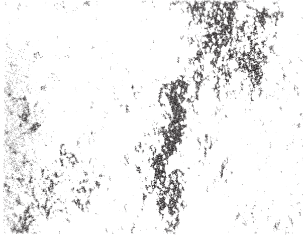
FIG. X1.57 Medium-Severity Raveling/Weathering
