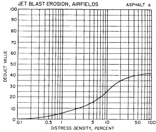
FIG. X3.6 Jet Blast
