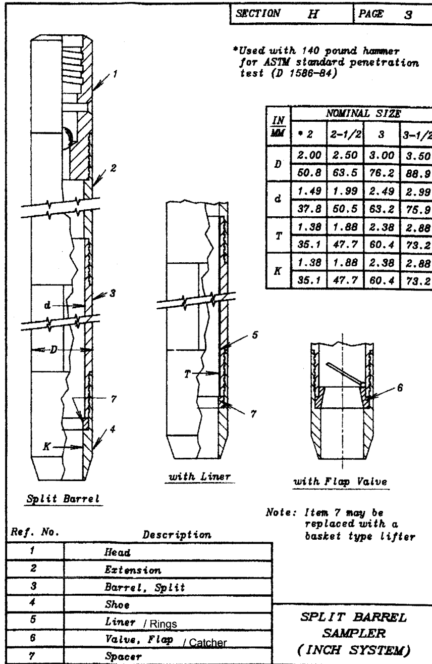
FIG. 1 Ring-Lined Barrel Sampling Assembly
