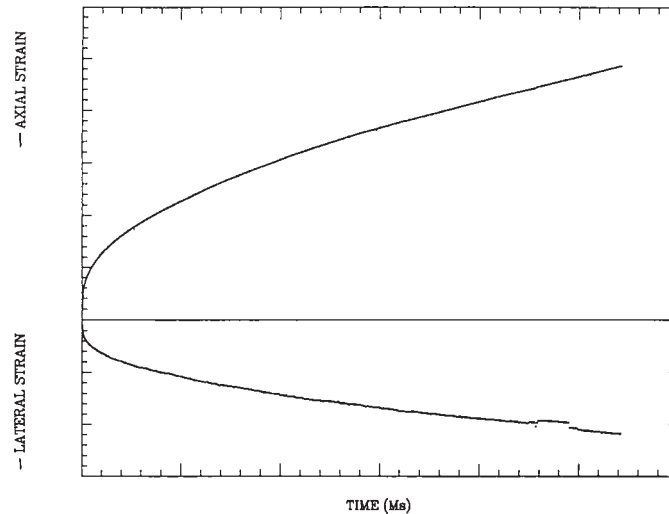
FIG. 1 Typical Strain-Versus-Time Curves
