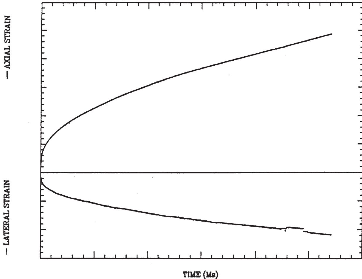
FIG. 1 Typical Strain-Versus-Time Curves
