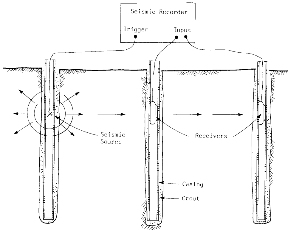
CROSS-SECTIONAL VIEW
