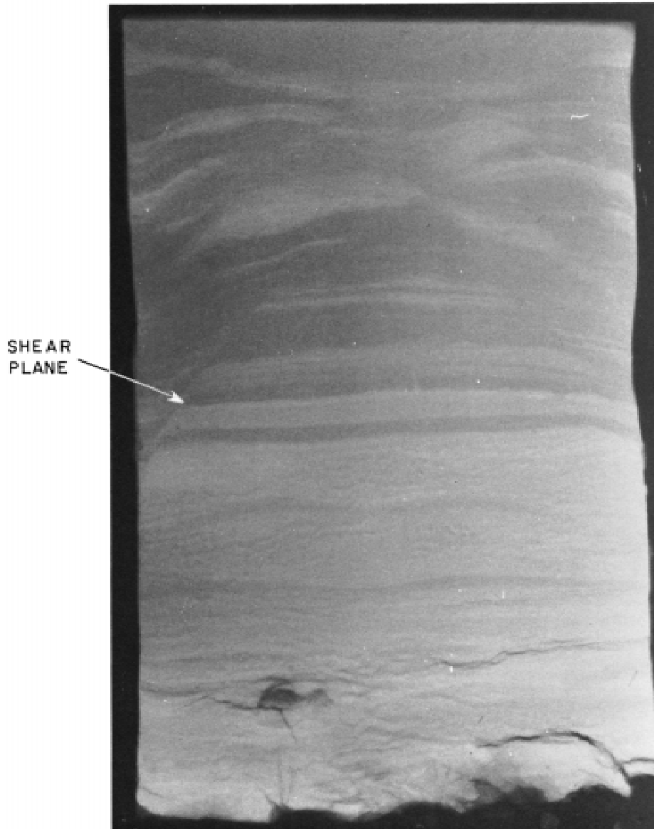
FIG. 12 Shear Fractures
