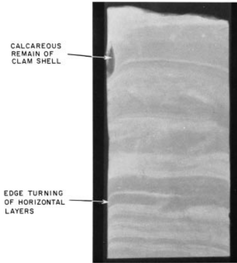
FIG. 10 Calcareous Concretions
