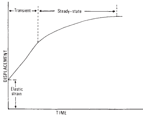
FIG. 5 Typical Creep Curve
