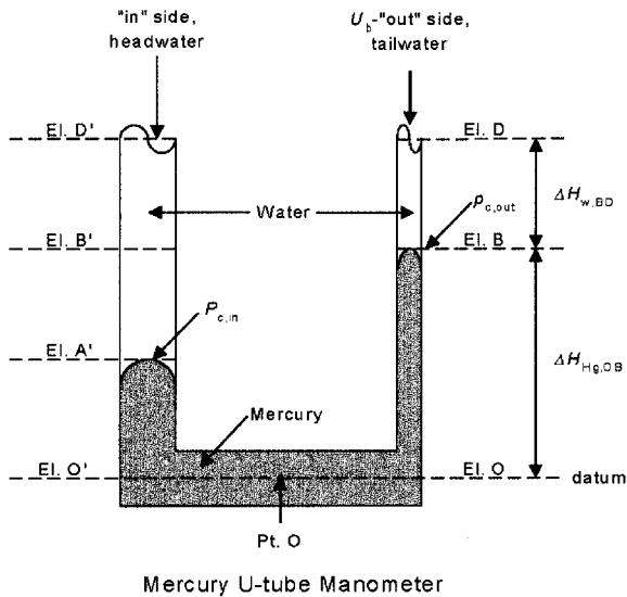
Mercury U-tube Manometer
