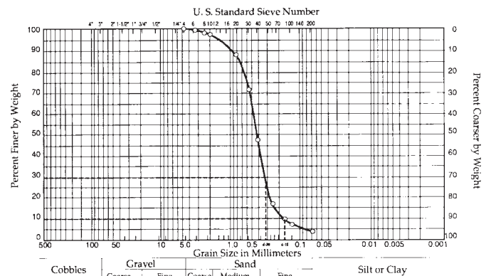
FIG. 1 Example Grading Curve for Design of Monitoring Well Screens
