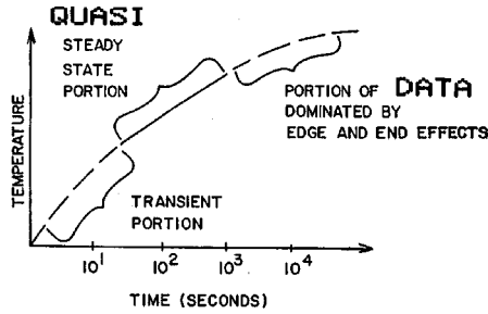
A) IDEALIZED CURVE FIG. 3 Typical Experimental Test Results Plotted on Semilog Graph
