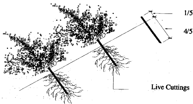
FIG. 2 Cross-Section of Live Stakes (Installed)
