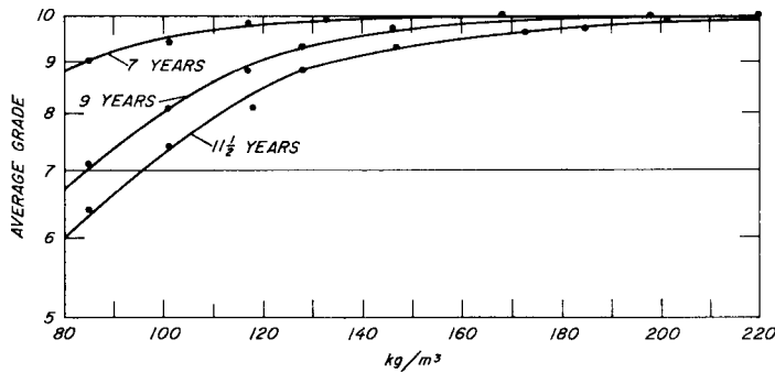
FIG. 2 Retention versus Grade; Dosage-Response Curves: Low Residue Coal Tar Creosote, Empty-Cell Treatment, 7, 9, and 11 1/2 Years in Test
