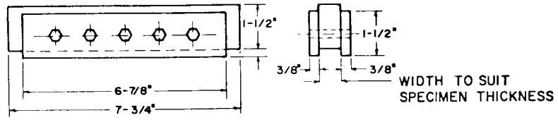
SPECIMEN LOADING BLOCKS 2 REQ'D
