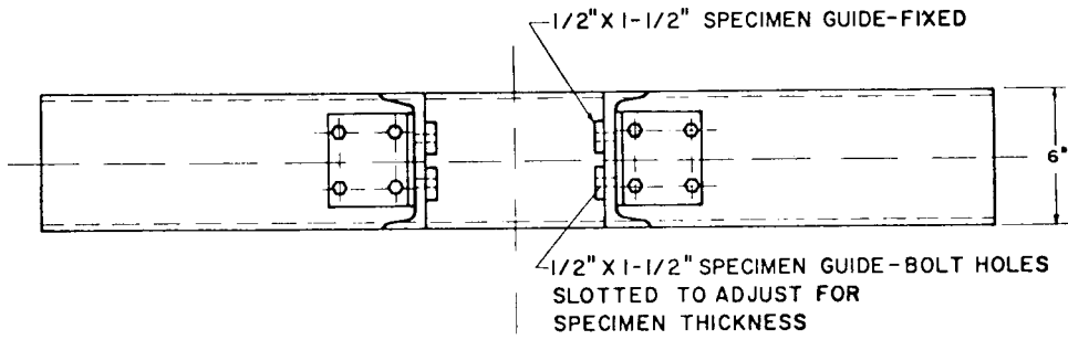
SPECIMEN LOADING BLOCKS 2 REQ'D
