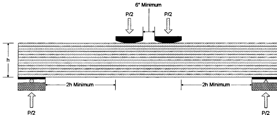
FIG. A7.1 Test Setup Based on Test Methods D 198 (not drawn to scale)
