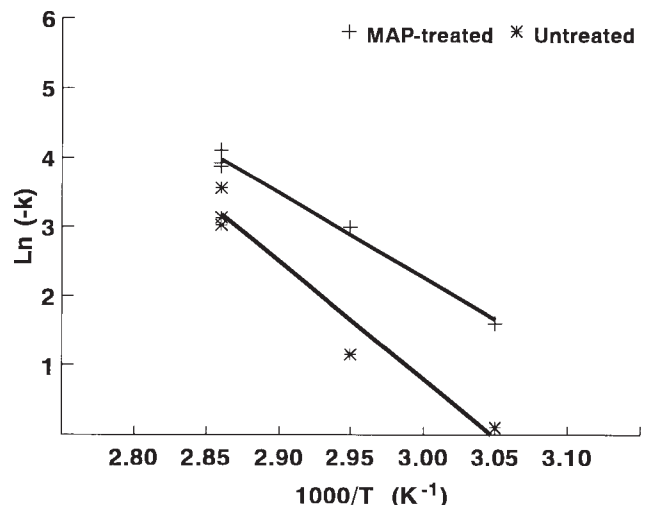
FIG. X1.2 Arrhenius Plot
