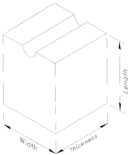
FIG. 1 Specimen Configuration
