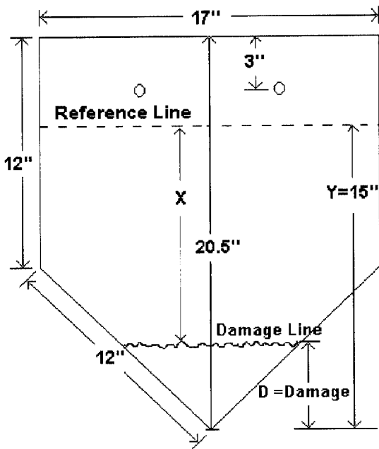
FIG. 3 Specimen and Measuring Diagram (Example)
