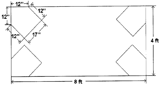
FIG. 2 Cutting Diagram
