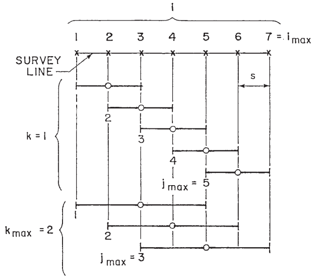
FIG. X1.1 Chord Positions
