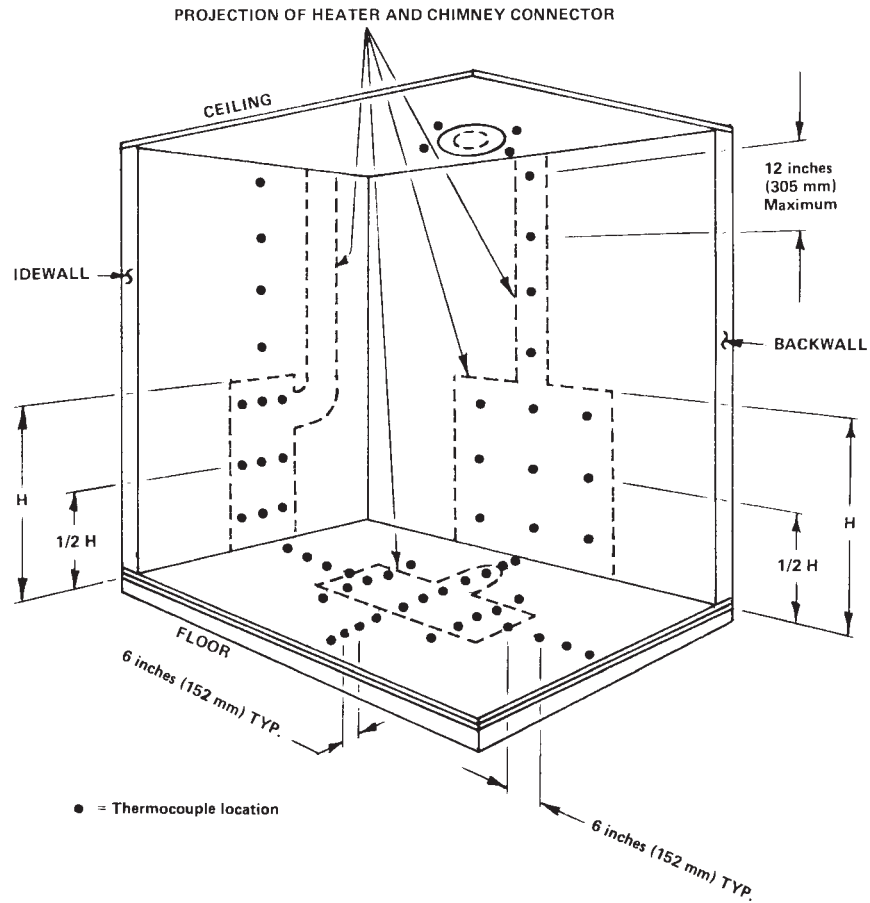
FIG. 6 Typical Thermocouple Locations for Walls and Floors of Test Structure (Right Wall Not Shown)
