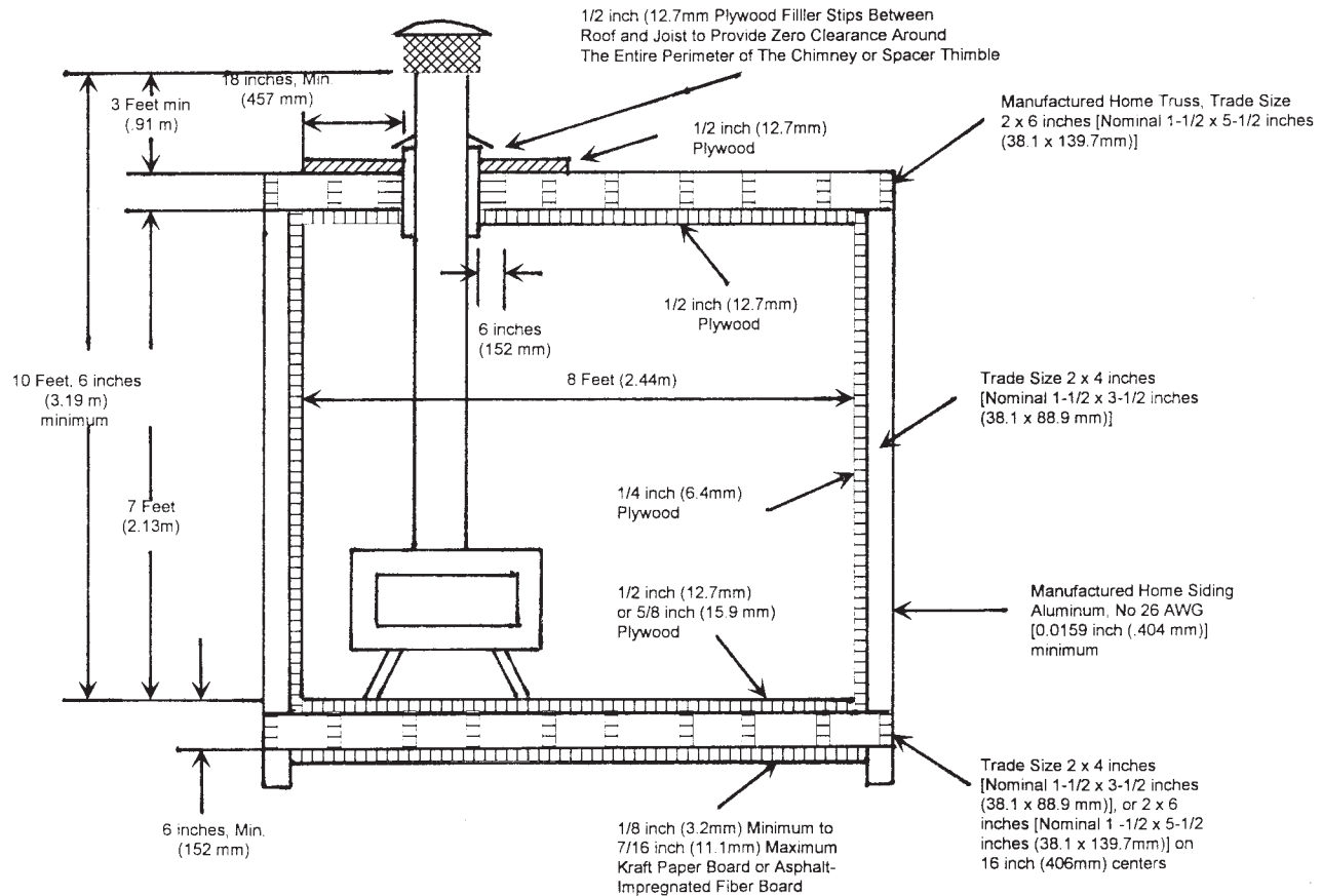
FIG. 2 Combined Conventional Home and Manufactured Home Test Structure; Installation with a Chimney or Type L Vertical Vent
