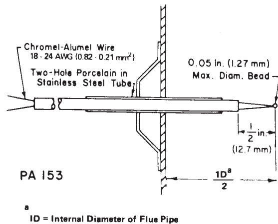
FIG. 4 Flue Gas Thermocouple and Support Bracket
