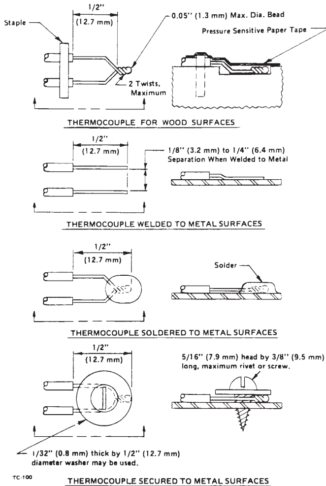
FIG. 5 Thermocouple Installation Methods
