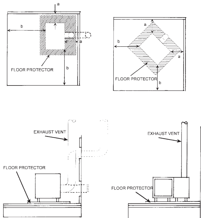
FIG. 3 Typical Fire Test Installations
