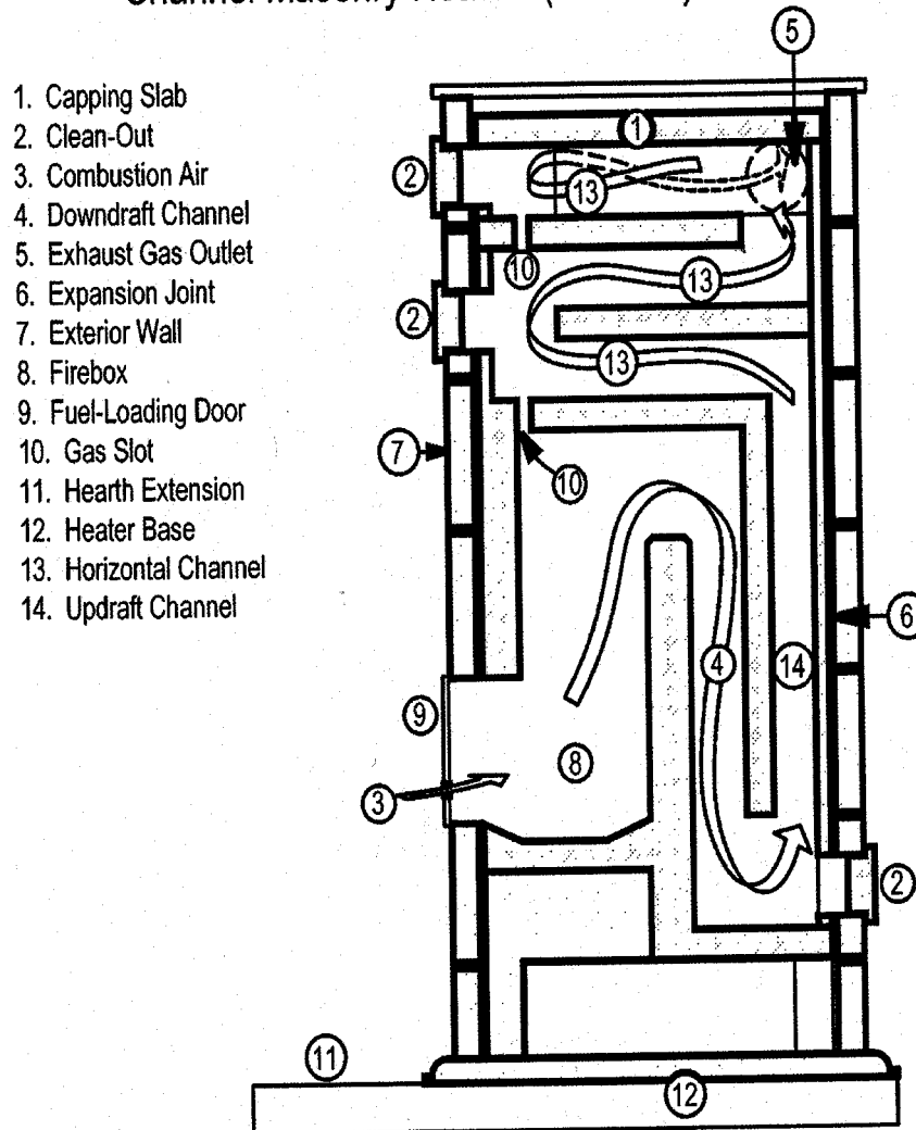
FIG. 3 Combination Vertical and Horizontal Channel Masonry Heater (German)
