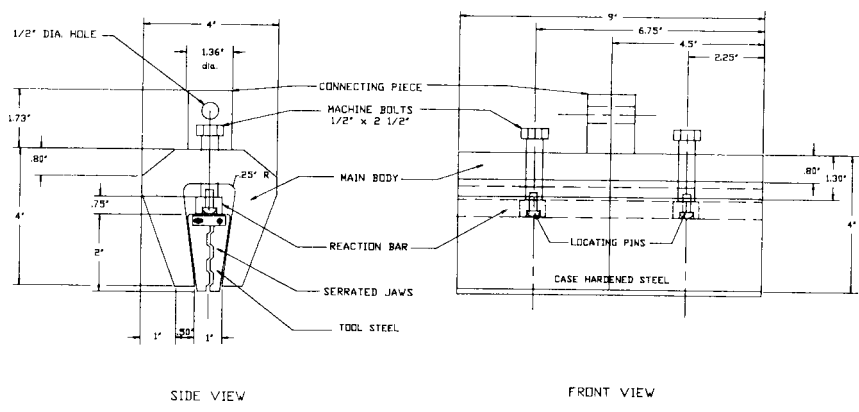
FIG. 4 Sanders Clamp
