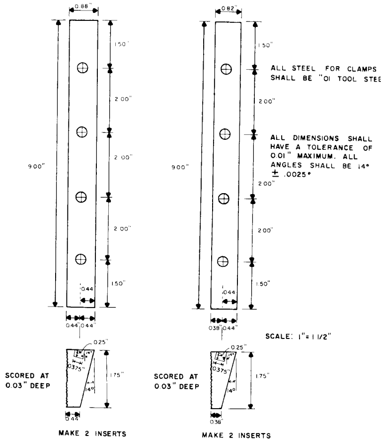
FIG. 2 Inserts for Wide Width Clamps
