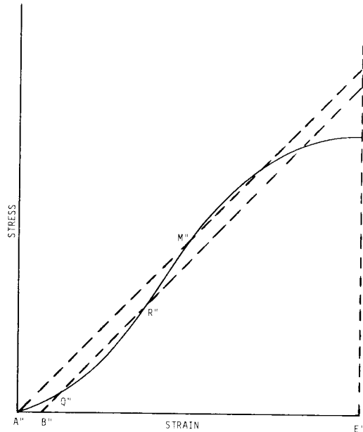
FIG. X3.1 Construction Line for Secant Modulus
