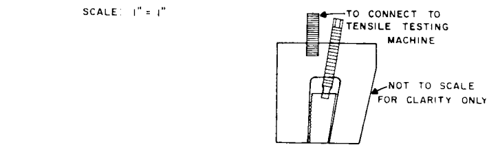
FIG. 3 End View of Composite of Clamp, Insert, and Threaded Rod
