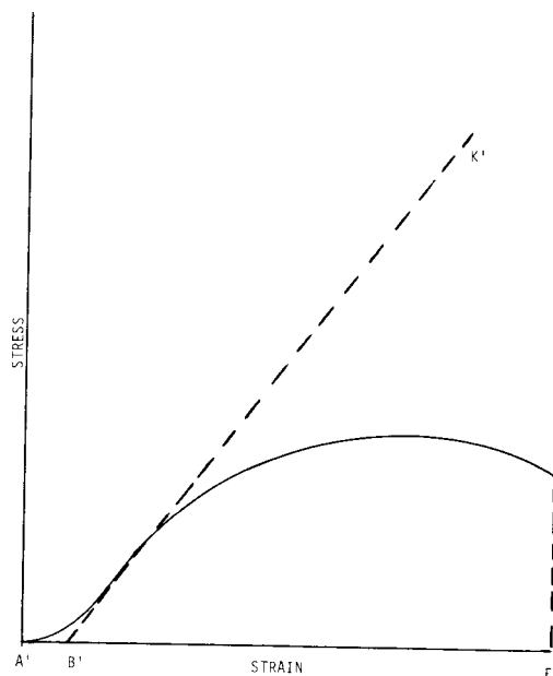
FIG. X2.1 Material with No Hookean Region
