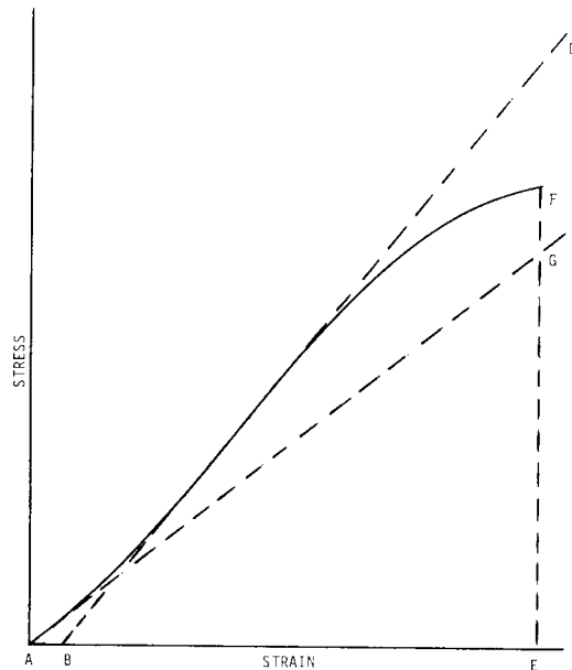
FIG. X1.1 Material with Hookean Region
