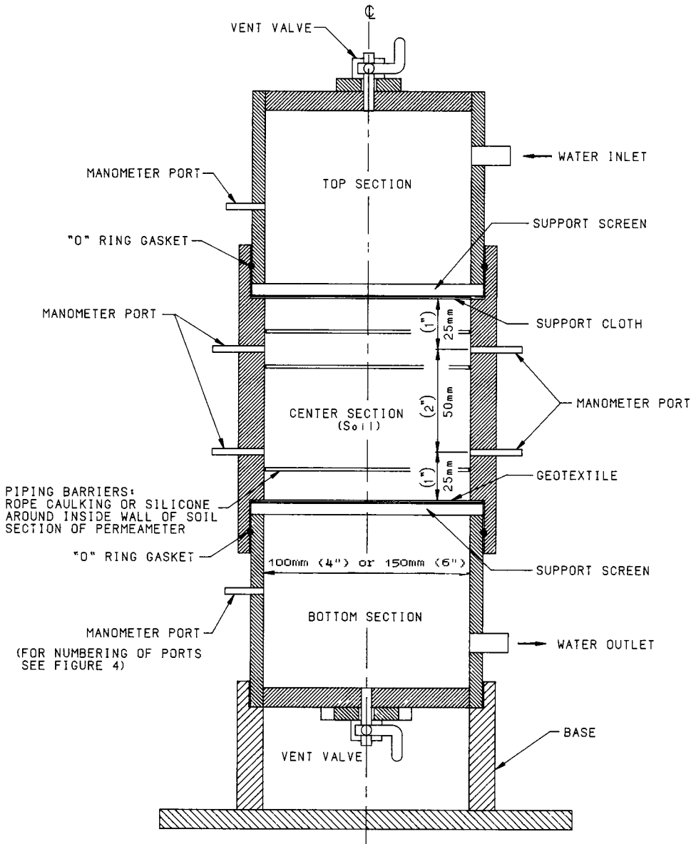
FIG. 2 Section—Geotextile Permeameter
