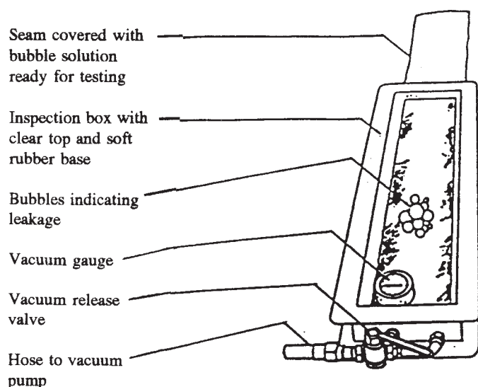
FIG. 1 Vacuum Chamber
